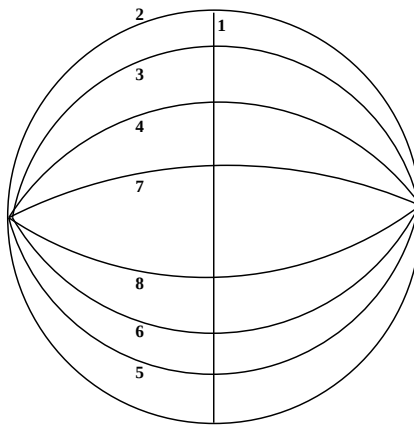
FIGURE 28 – Arrangement of pseudolines obtained from Exemple 2.
