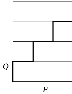
FIGURE 21 – Lattice paths P and Q
